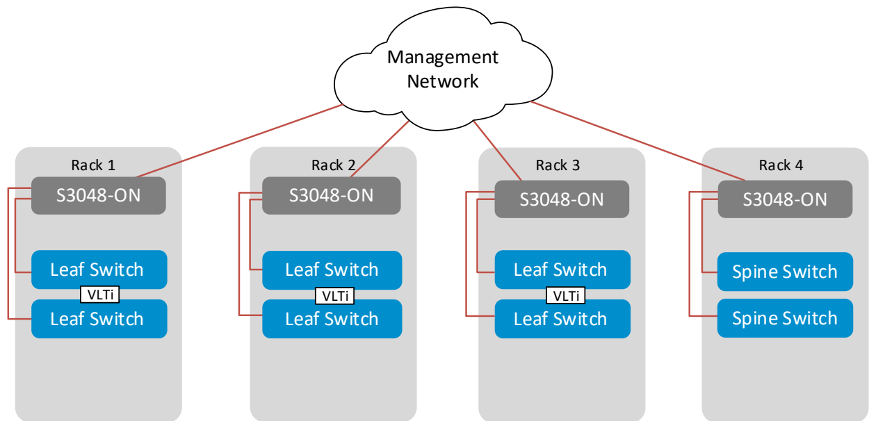
Figure 9 Management Network
