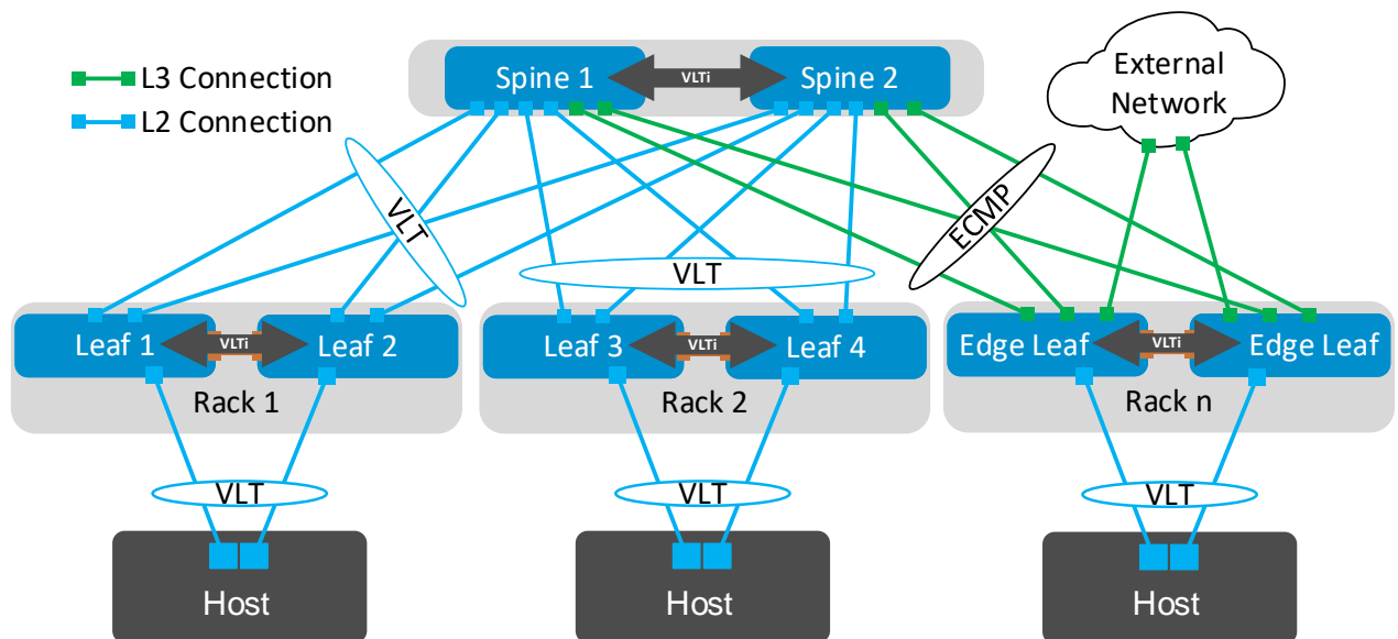
Figure 8 Layer 2 leaf-spine network
