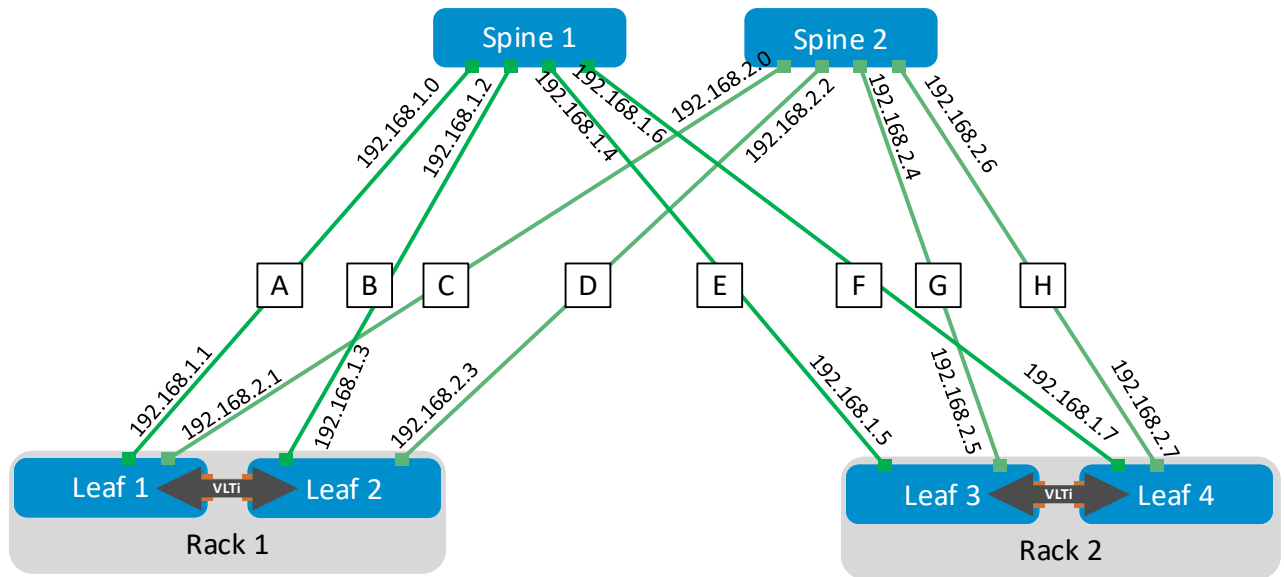
Figure 13 Point-to-point IP addresses
